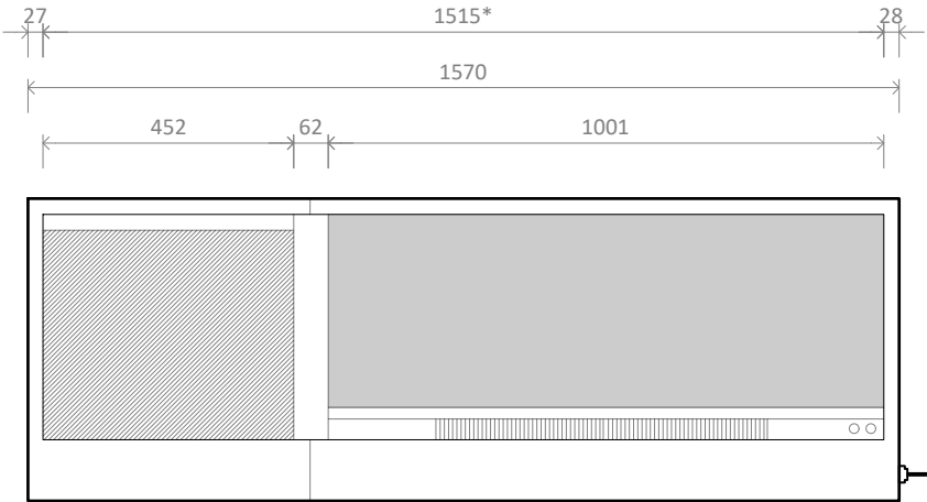
LE/LR1000 MK2 with Single Niche Left - Front
