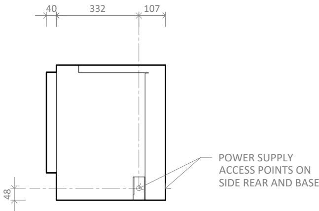
LE/LR1000 MK2 with Single Niche Right - Side
