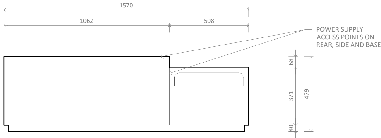
LE/LR1000 MK2 with Single Niche Right - Plan
