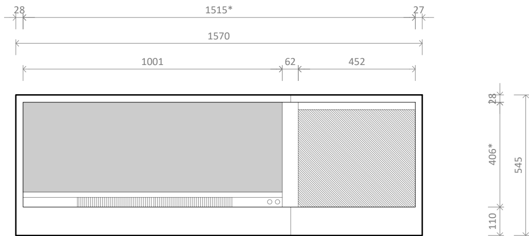
LE/LR1000 MK2 with Single Niche Right - Front
