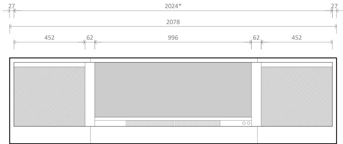
LE/LR1000 MK2 with Double Niche - Front
