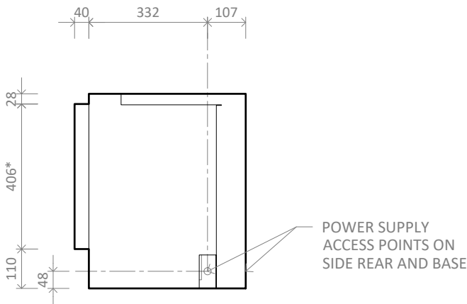
LE/LR1000 MK2 with Double Niche - Side R
