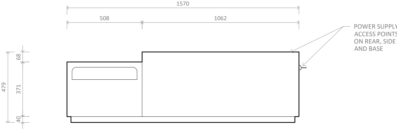
LE/LR1000 MK2 with Single Niche Left - Plan
