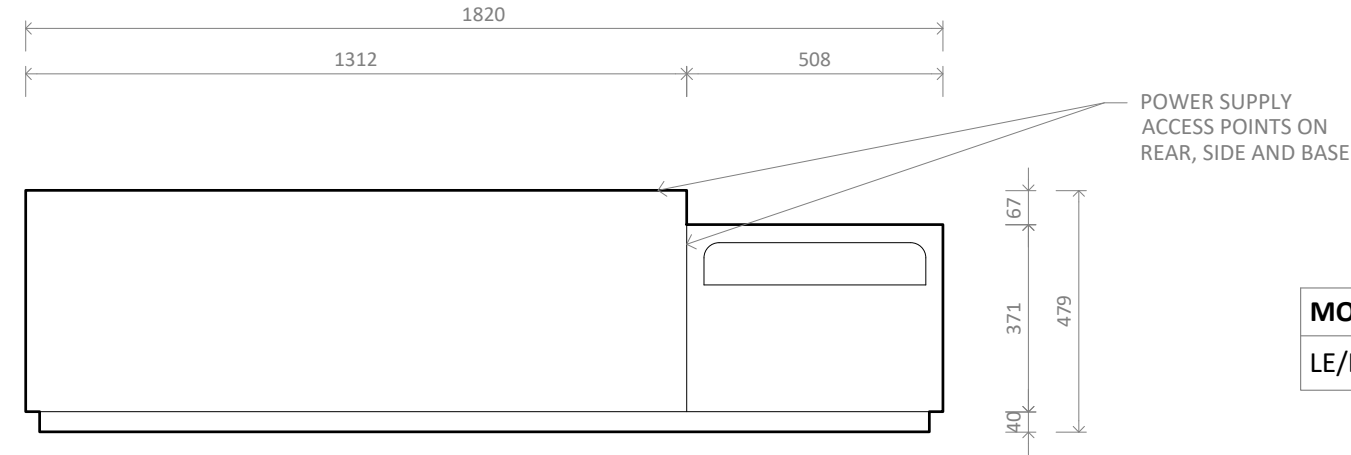
LE/LR1250 MK2 with Single Niche Right - Plan
