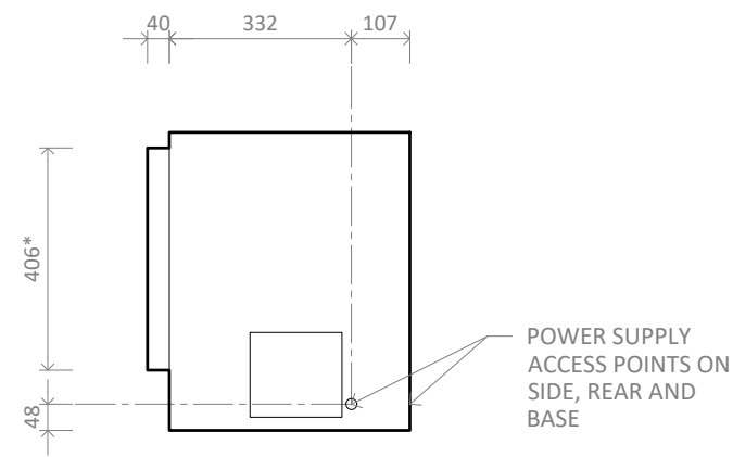
LE/LR1250 MK2 - Side
