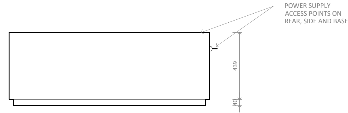
LE/LR1250 MK2 - Plan
