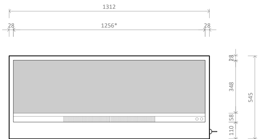
LE/LR1250 MK2 - Front
