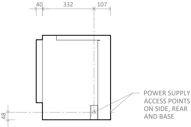
LE/LR1250 MK2 with Single Niche Right - Side
