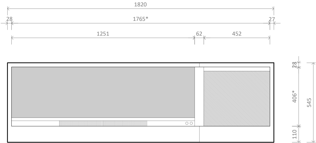
LE/LR1250 MK2 with Single Niche Right - Front
