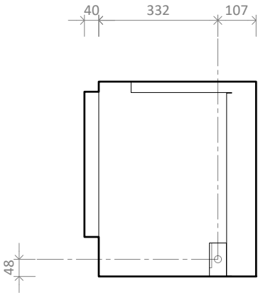
LE/LR1250 MK2 with Double Niche - Side R
