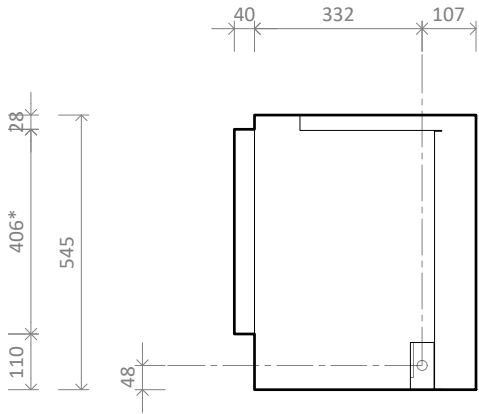
LE/LR1550 MK2 with Double Niche - Side R
