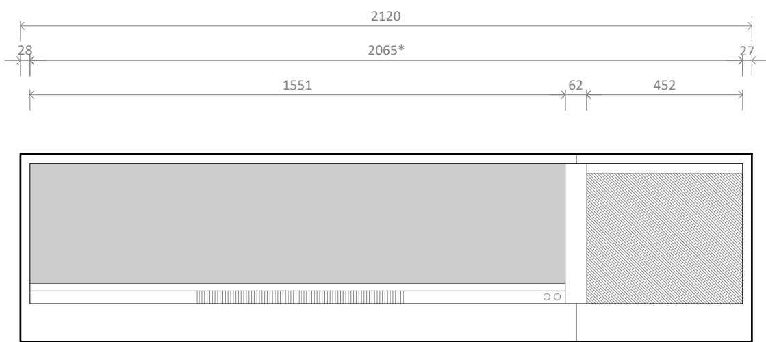
LE/LR1550 MK2 with Single Niche Right - Front
