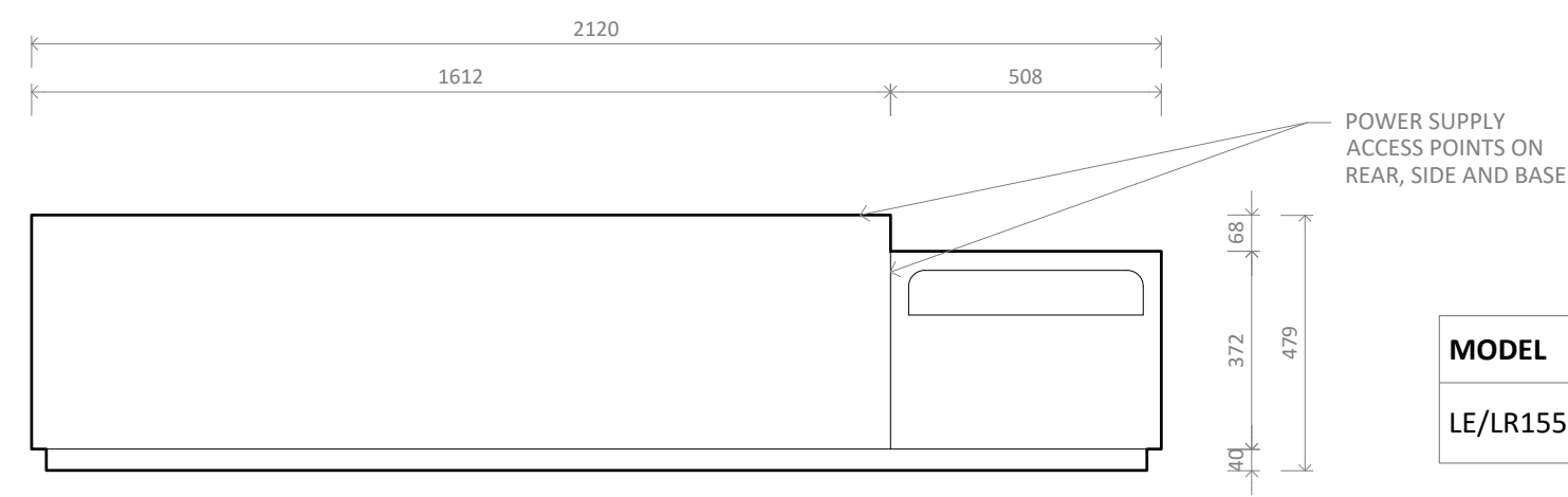
LE/LR1550 MK2 with Single Niche Right - Plan
