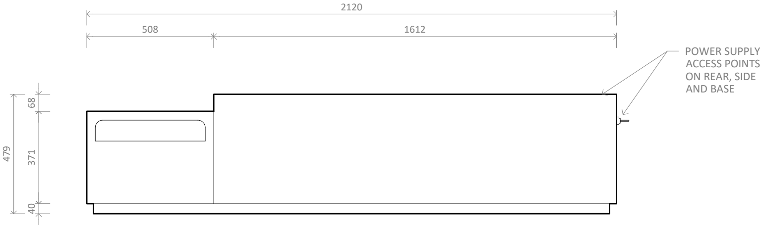
LE/LR1550 MK2 with Single Niche Left - Plan
