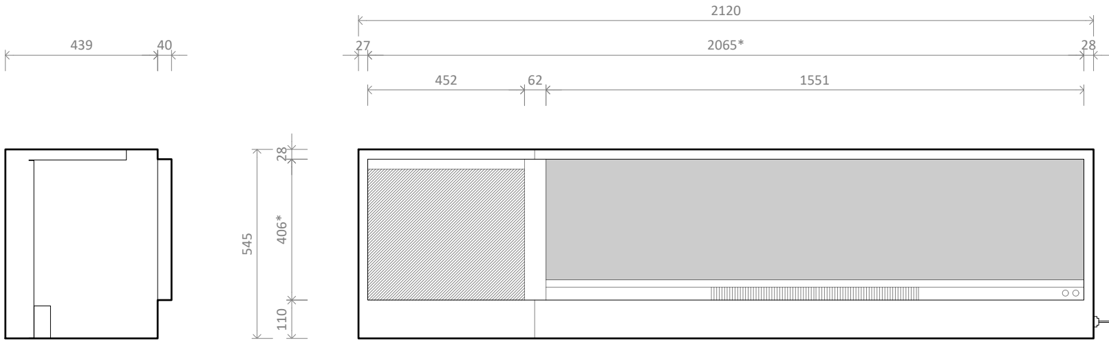
LE/LR1550 MK2 with Single Niche Left - Side
