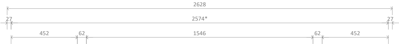
LE/LR1550 MK2 with Double Niche - Plan
