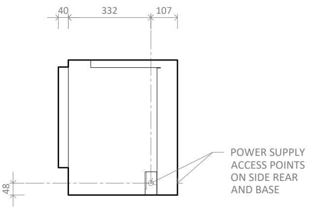
LE/LR1550 MK2 with Single Niche Right - Side
