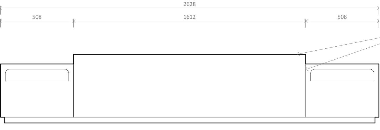
LE/LR1550 MK2 with Double Niche - Plan
