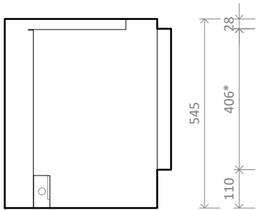
LE/LR1750 MK2 with Single Niche Left - Side
