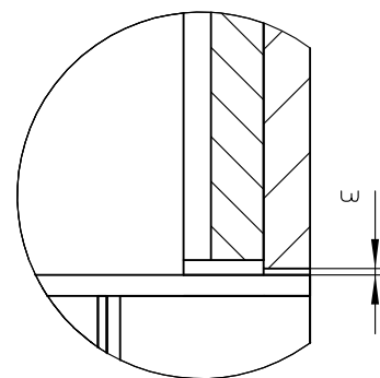
Detail1 SCALE 1:4
