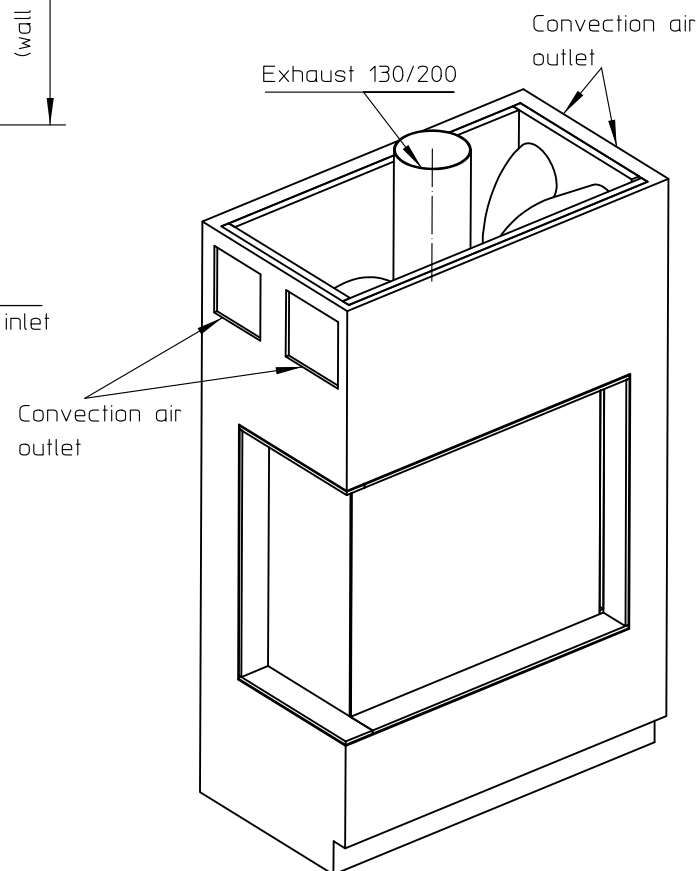
Detail1 SCALE 1:4
