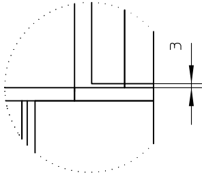
Detail1 SCALE 1:4
