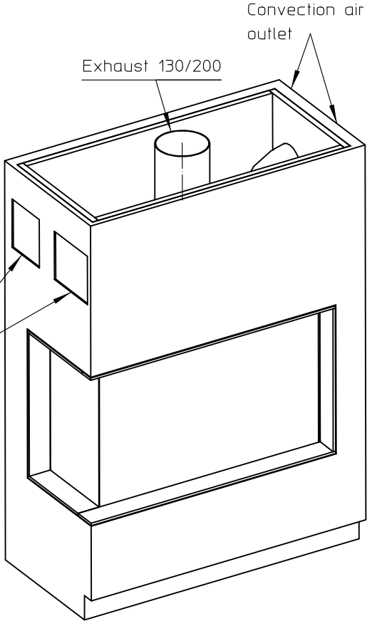
Detail1 SCALE 1:4
