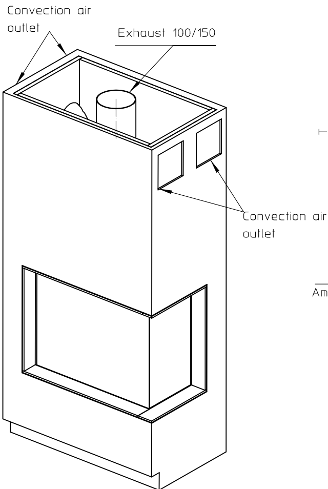
Detail2 SCALE 1:4
