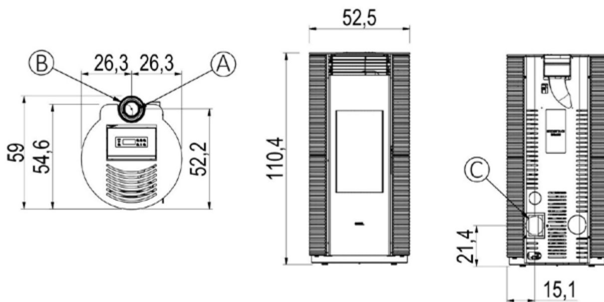
Fig. 12 - General dimensions: Spin Plus 9 Up-Twin T1
