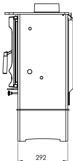
Side
