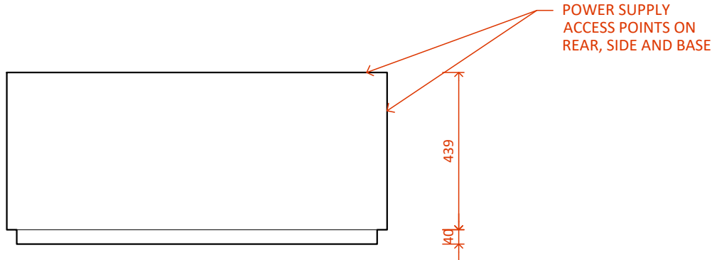
LE1000 MK2 - Plan
