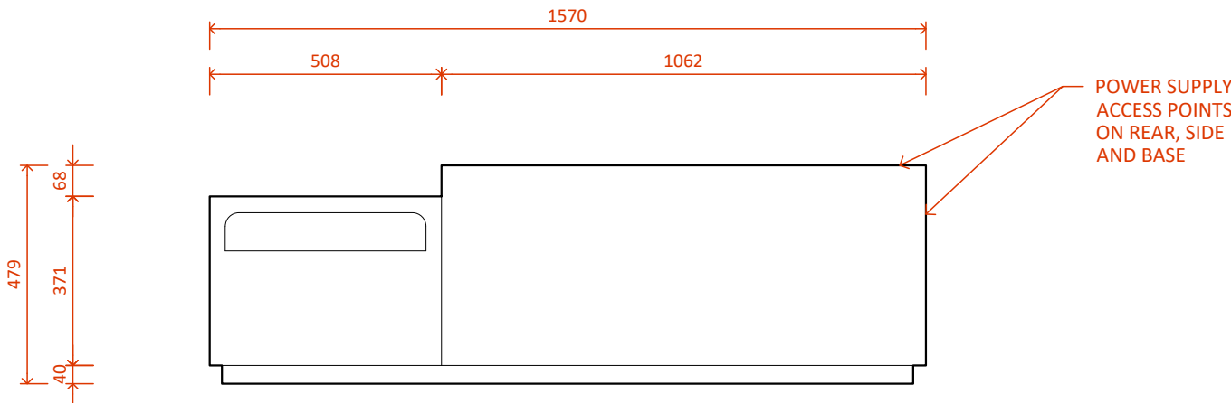
LE1000 MK2 with Single Niche Left - Plan
