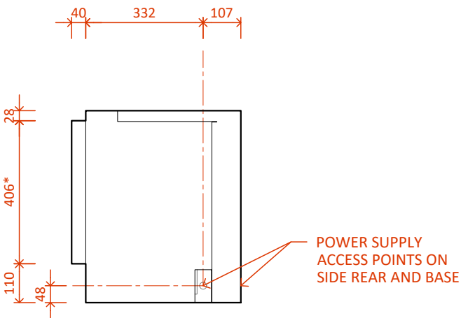
LE1000 MK2 with Double Niche - Side R
