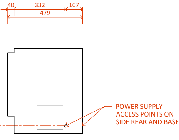
LE1000 MK2 - Side
