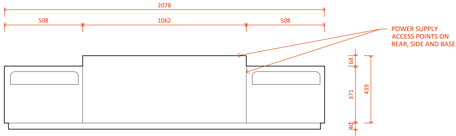
LE1000 MK2 with Double Niche - Plan
