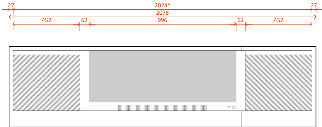
LE1000 MK2 with Double Niche - Front
