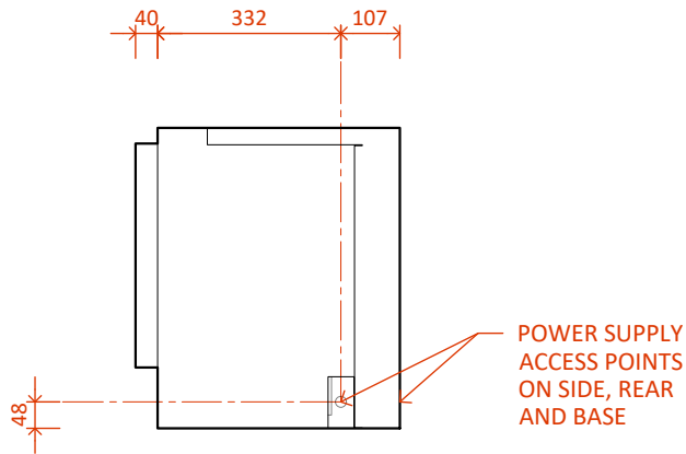
LE1250 MK2 with Single Niche Right - Side
