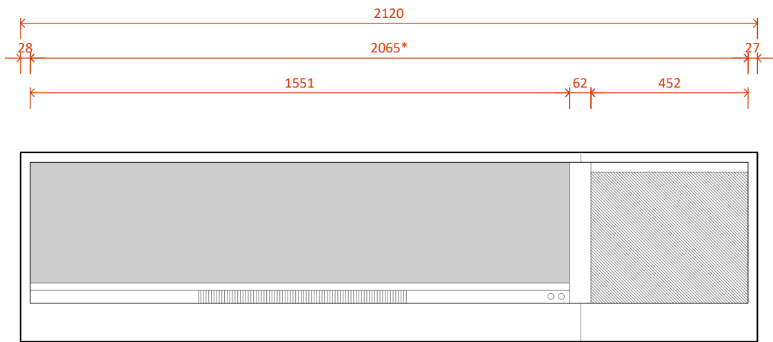
LE1550 MK2 with Single Niche Right - Front
