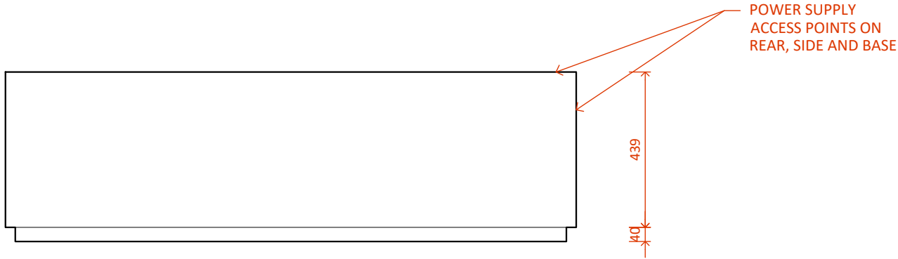
LE1550 MK2 - Plan
