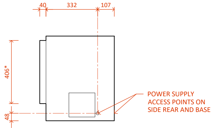
LE1550 MK2 - Side
