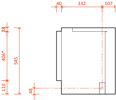
LE1550 MK2 with Double Niche - Side R
