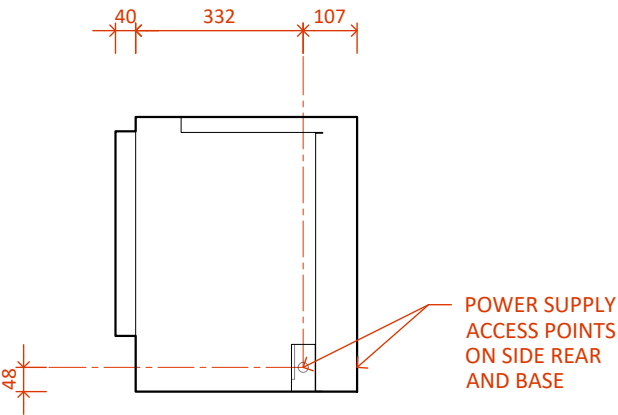
LE1550 MK2 with Single Niche Right - Side
