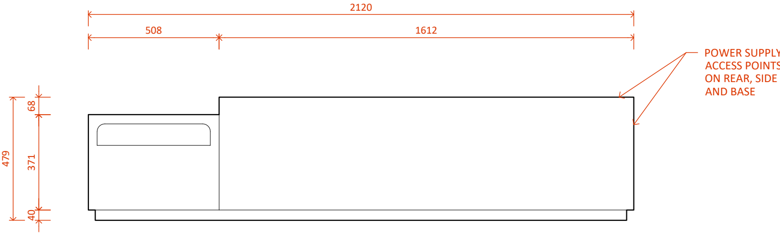
LE1550 MK2 with Single Niche Left - Plan
