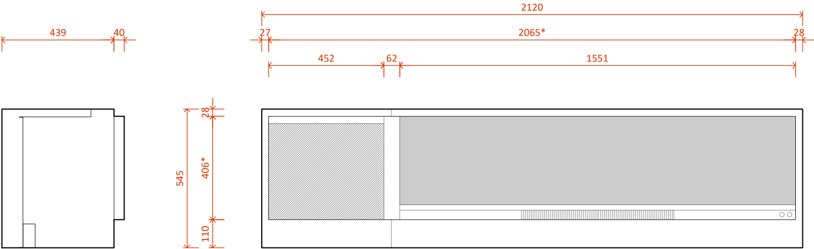
LE1550 MK2 with Single Niche Left - Side
