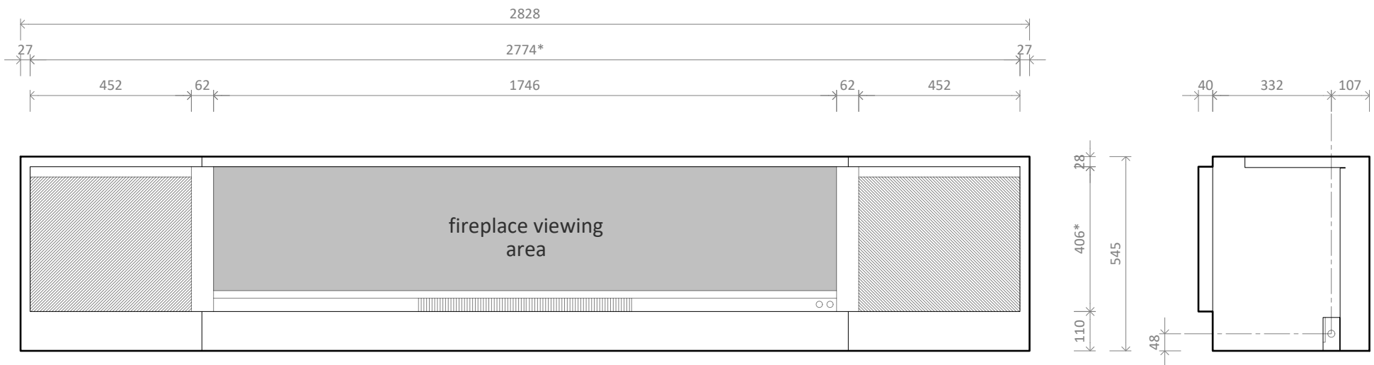
LE/LR1750 MK2 with Double Niche - Front
