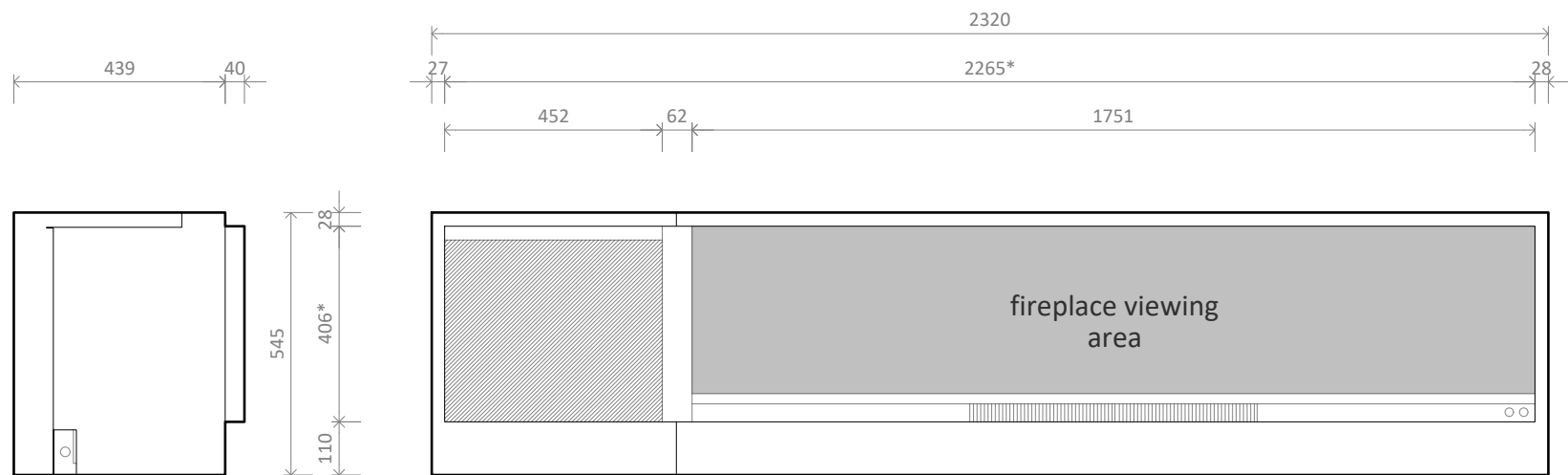
LE/LR1750 MK2 with Single Niche Left - Side
