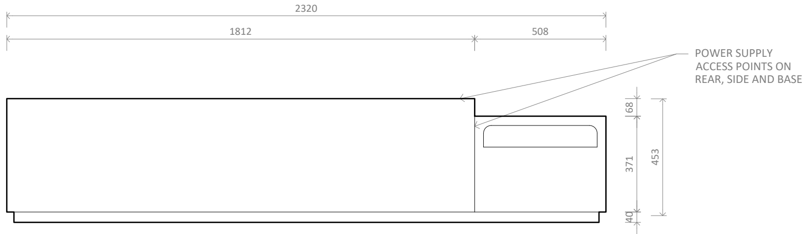
LE/LR1750 MK2 with Single Niche Right - Plan
