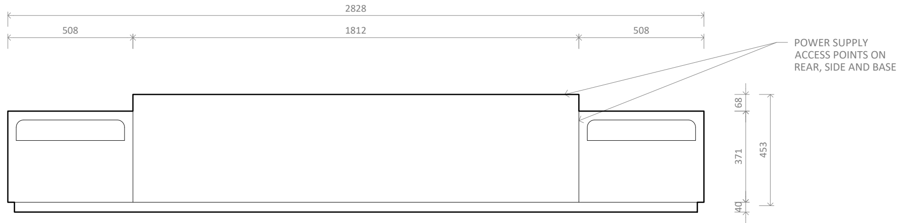
LE/LR1750 MK2 with Double Niche - Plan
