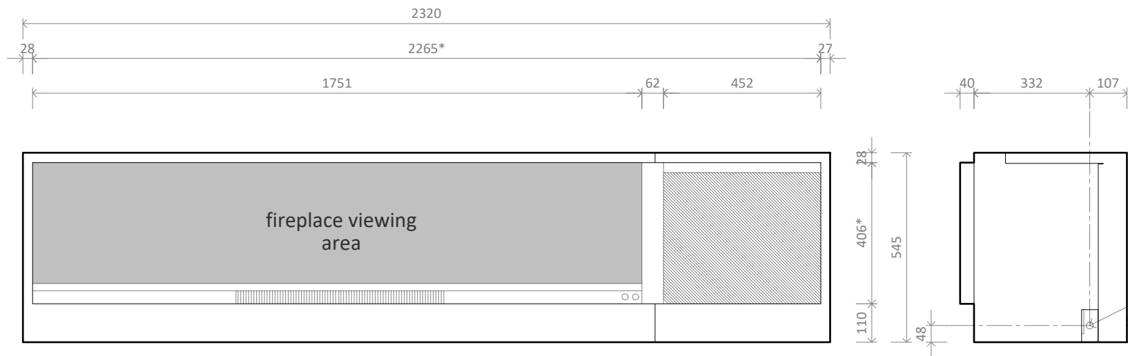
LE/LR1750 MK2 with Single Niche Right - Front
