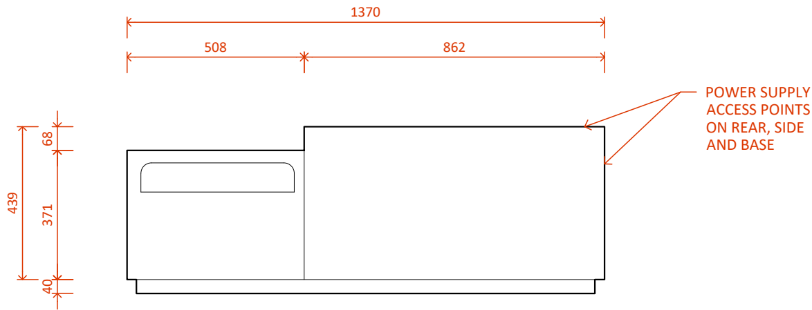
LE800 MK2 with Single Niche Left - Plan
