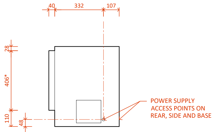
LE800 MK2 - Side
