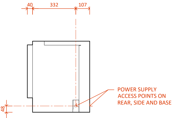
LE800 MK2 with Single Niche Right - Side
