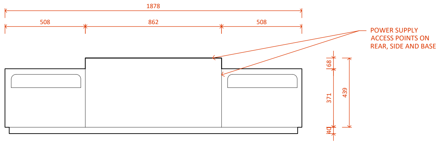
LE800 MK2 with Double Niche - Plan
