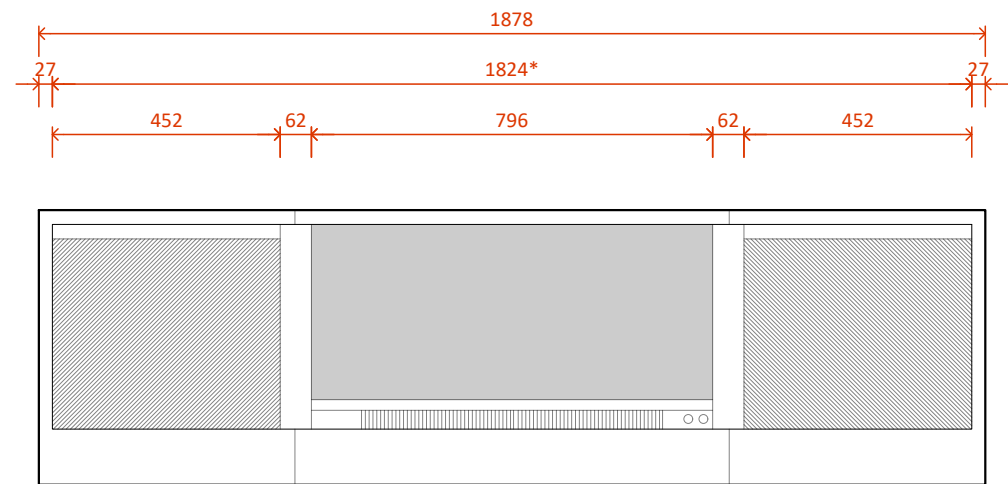
LE800 MK2 with Double Niche - Front
