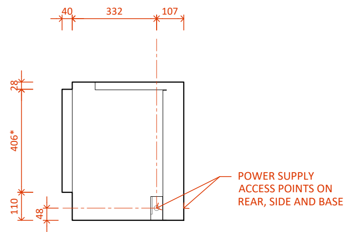
LE800 MK2 with Double Niche - Side R
