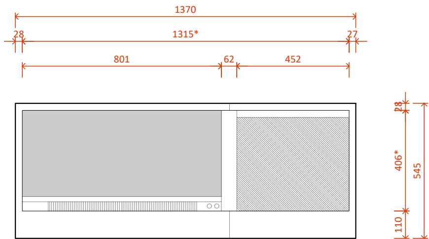
LE800 MK2 with Single Niche Right - Front
