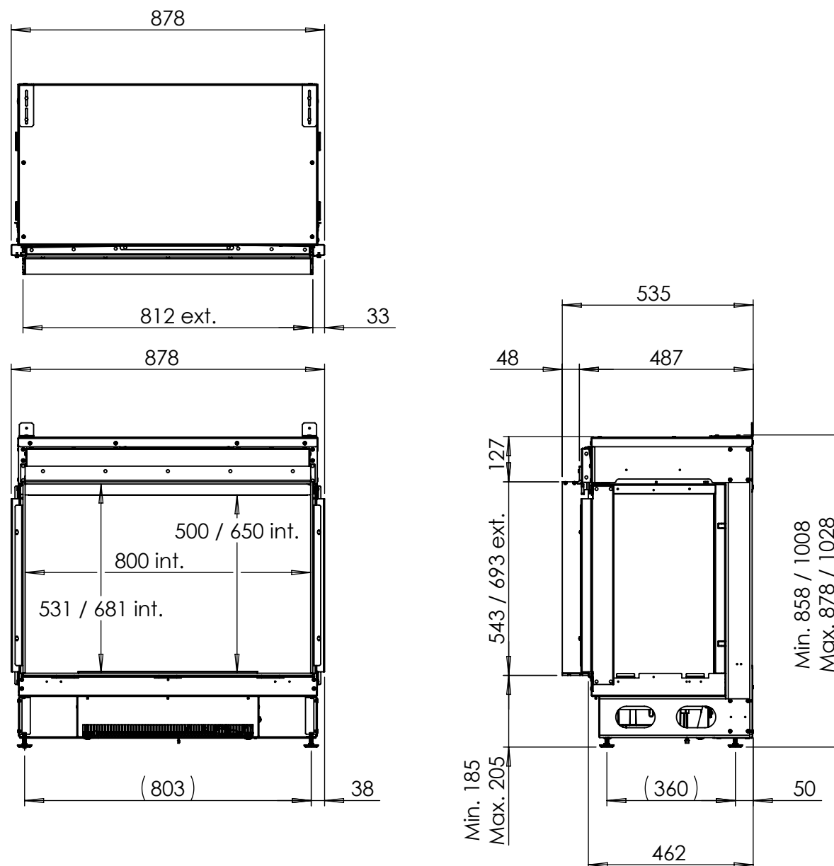
Dimensional Drawing e-MatriX 800x500 I + 800/650 I (MkII)
