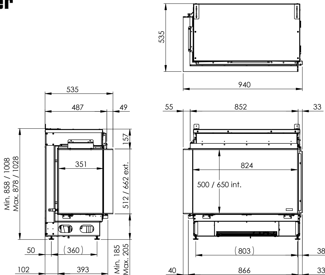
Dimensional Drawing e-MatriX 800/500 IIL + 800/650 IIL (MkII)
