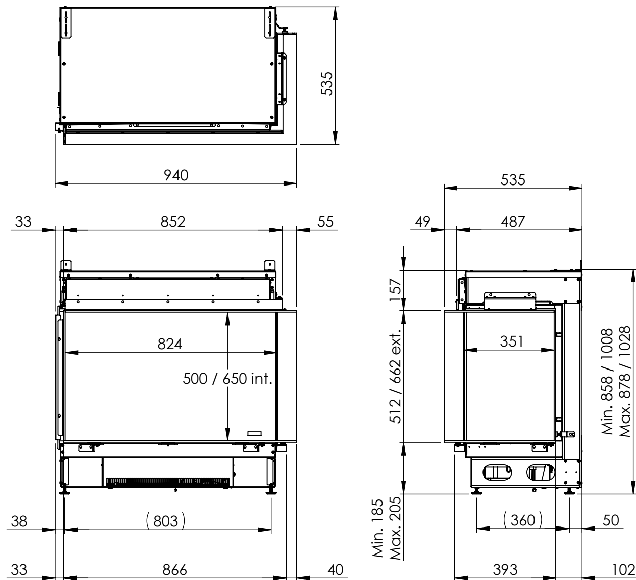
Dimensional Drawing e-MatriX 800x500-650 IIR (MkII)
