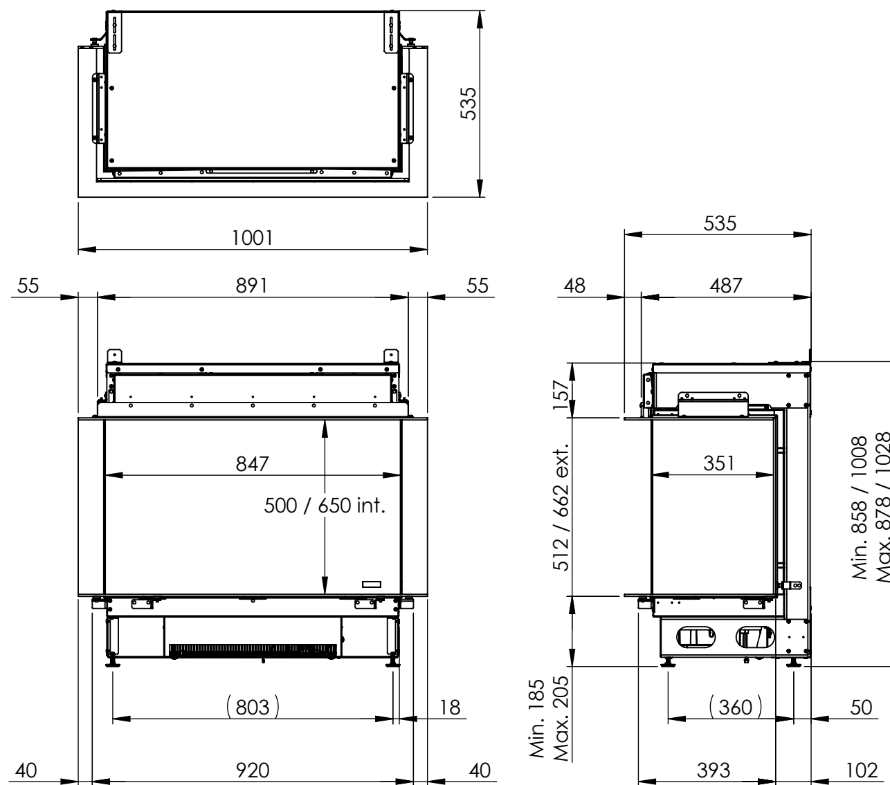
Dimensional Drawing e-MatriX 800/500 III + e-MatriX 800/650 III (MkII)
