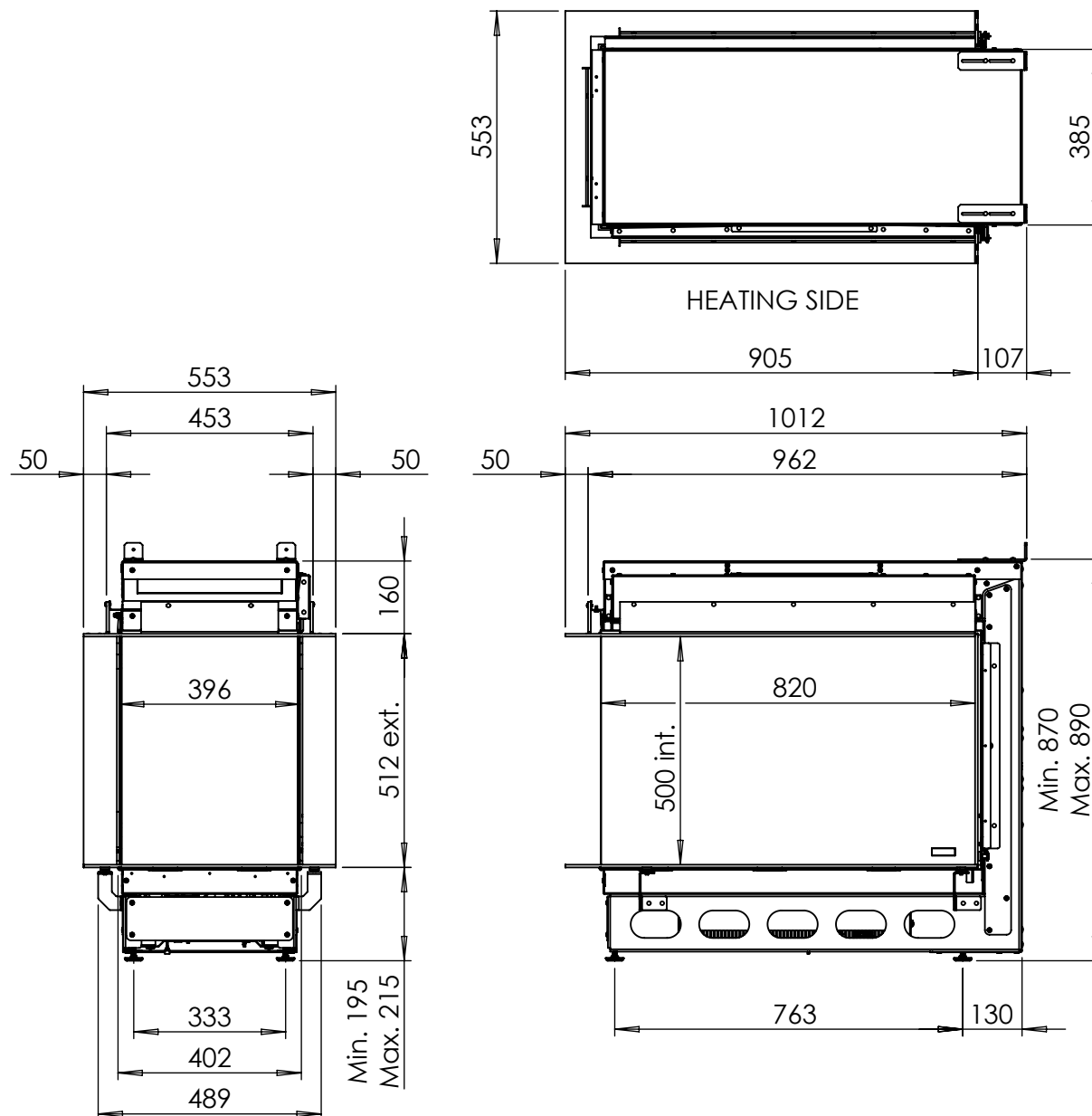
Dimensional Drawing e-MatriX heat 800x500 RD (MkII)
