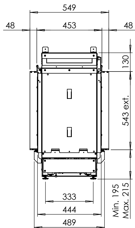
Dimensional Drawing e-MatriX heat 800x500 ST (MkII)
