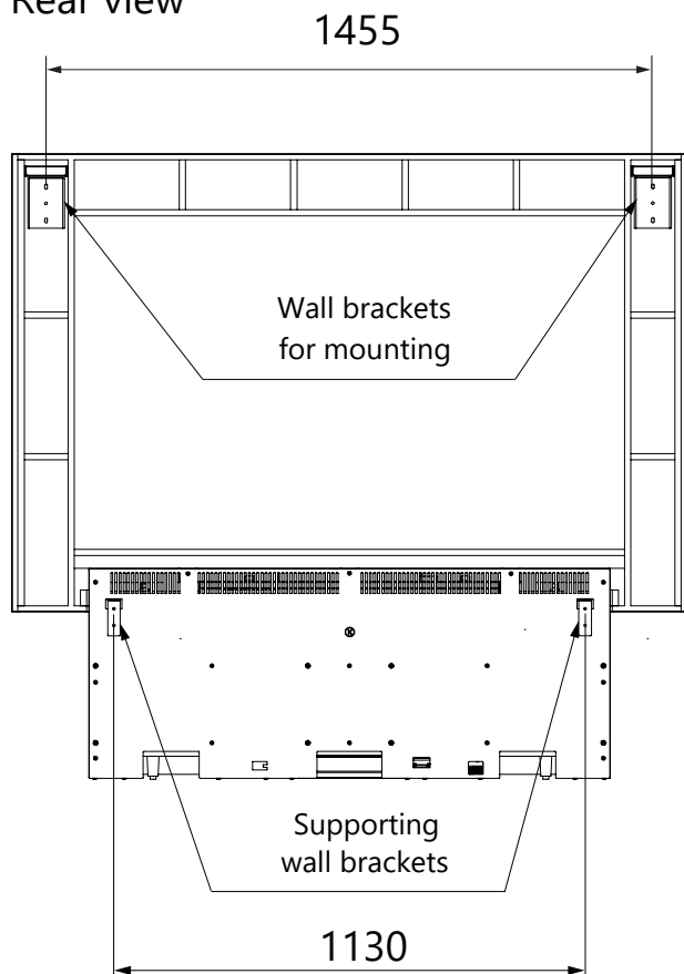
Rear view
