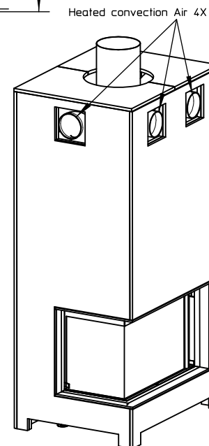
Detail2 Scale 1:5
