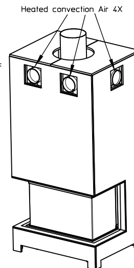
Detail2 Scale 1:5
