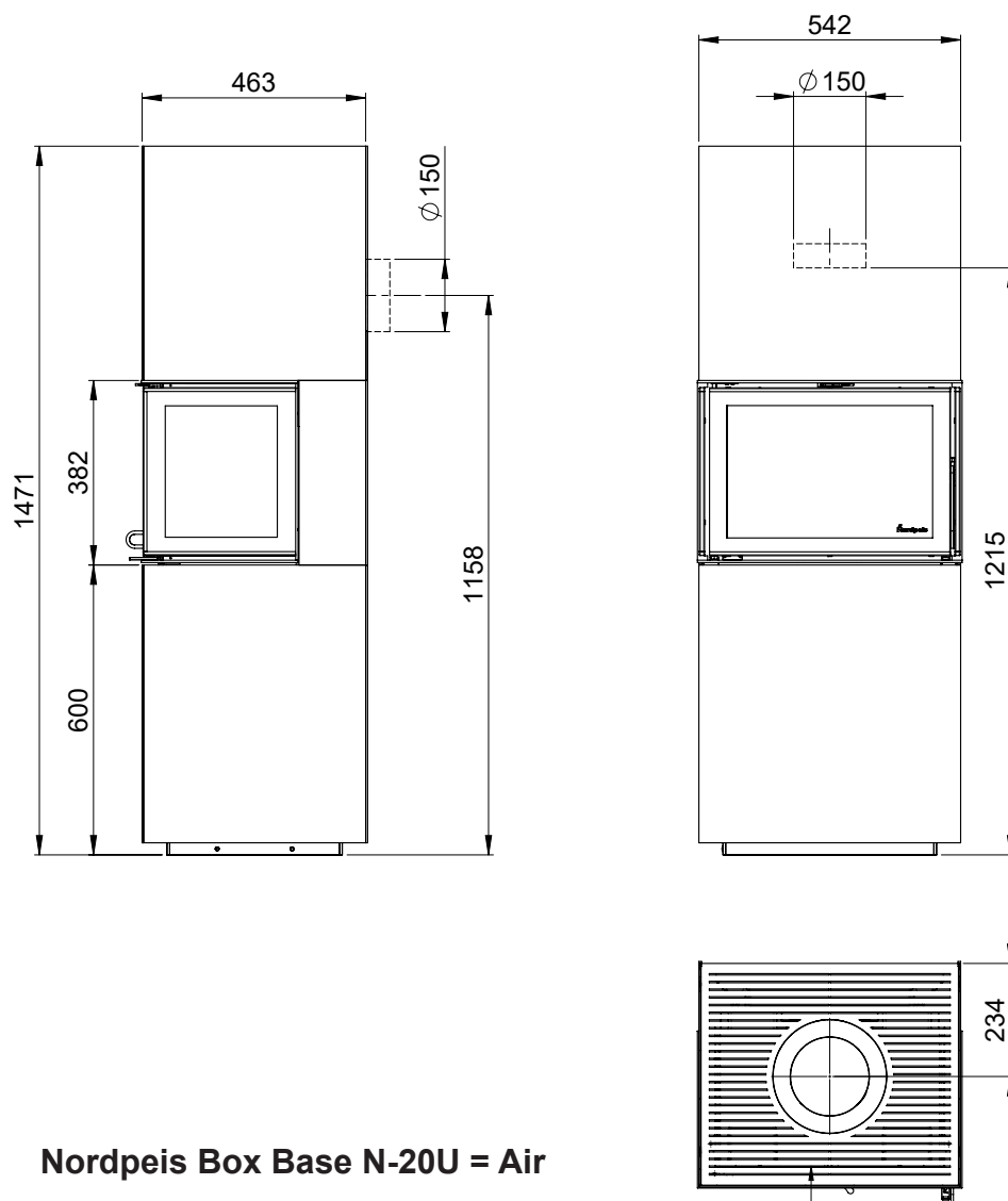
Nordpeis Box Base N-20U = mm / Chimney connections
